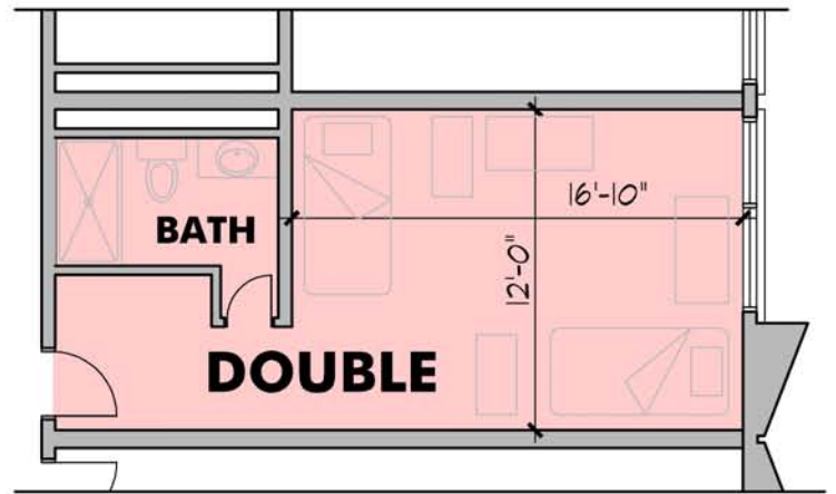
TYPICAL BEDROOM
